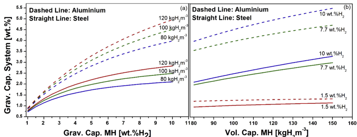
Fig. 12 – (a) Gravimetric capacity of the system as a function of the gravimetric capacity of MH, using a volumetric capacity of MH equal to 80–100–120 kgH 2 m -3 (b) Gravimetric capacity of the system as a function of the volumetric capacity of the MH, using a gravimetric capacity of MH of 1.5–7.7–10 wt.% H 2 . In both cases, it was considered a diameter of tube of 10 cm in aluminium (dashed line) and steel (straight line).
