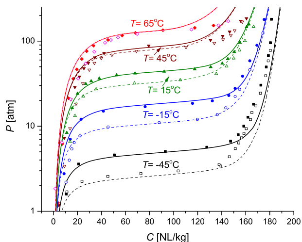
Fig. 8 – Experimental (points) and calculated (lines) isotherms (solid lines/filled symbols for H absorption; dashed lines/empty symbols for H desorption) for C14–Ti 0.7 Zr 0.3 (Cr,Fe,Mn,Ni) 2 (V. Yartys and M. Lototskyy, unpublished data). Parameters of the calculated isotherms listed in Table 3 were obtained by the fitting of the experimental data using model [100].
