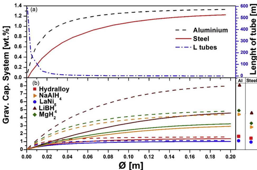
Fig. 13 – The gravimetric capacity of the system as a function of the diameter of tube. (a) Curves have been obtained considering a MH with a gravimetric and volumetric capacity of 1.5 wt.% H 2 and 100 kgH 2 m -3 , respectively. The gravimetric capacity of the system is calculated for aluminium (dashed line) and steel (straight line) tube. It is also reported in dashed dot line the variation of the length of tube as a function of the diameter. (b) The gravimetric capacity of the system is reported considering different hydrides.
