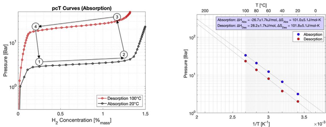
Fig. 1 – Working principles of the metal hydrides hydrogen compressor (left) and van 't Hoff plot for a typical AB 5 alloy (from Ref. [85]).
